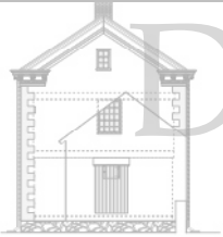
EXTERIOR ELEVATION - NORTH
